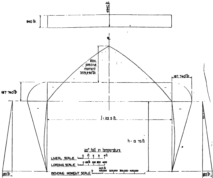
Fig. 117.—Maximum Positive Bending Moment.
